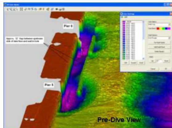
Figure N-3. On left, initial plan of multibeam survey at Mel Price Lock & Dam (Mississippi River). Significant scour (15 to 20 ft below normal grade) was indicated at piers 5, 6, 9, and 10). On right, 3D detail model of Pier 5 and 6 scour area furnished to divers. (St. Louis District)
