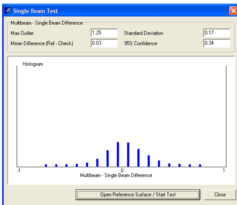
Figure F-6. Shuman Multibeam vs. S/V Cherneski Single Beam: Single beam 0.03' shaller.
