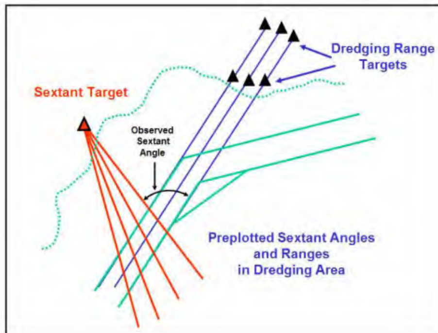
Figure G-2. Hopper dredge control using combined visual ranges and sextant angles.
